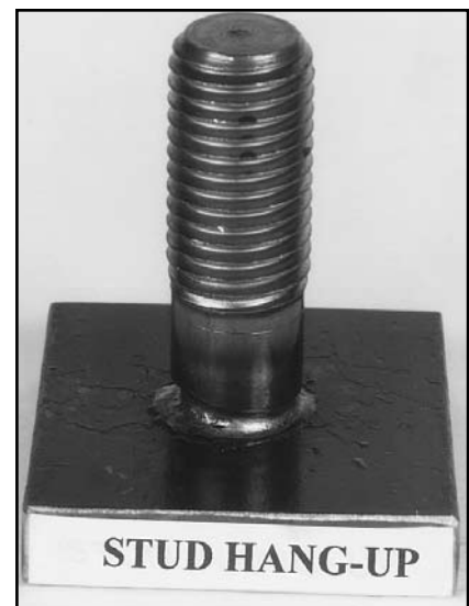
Fig. 12. Visual inspection of stud weld appearance. Source: Nelson Stud Welding, Inc.
