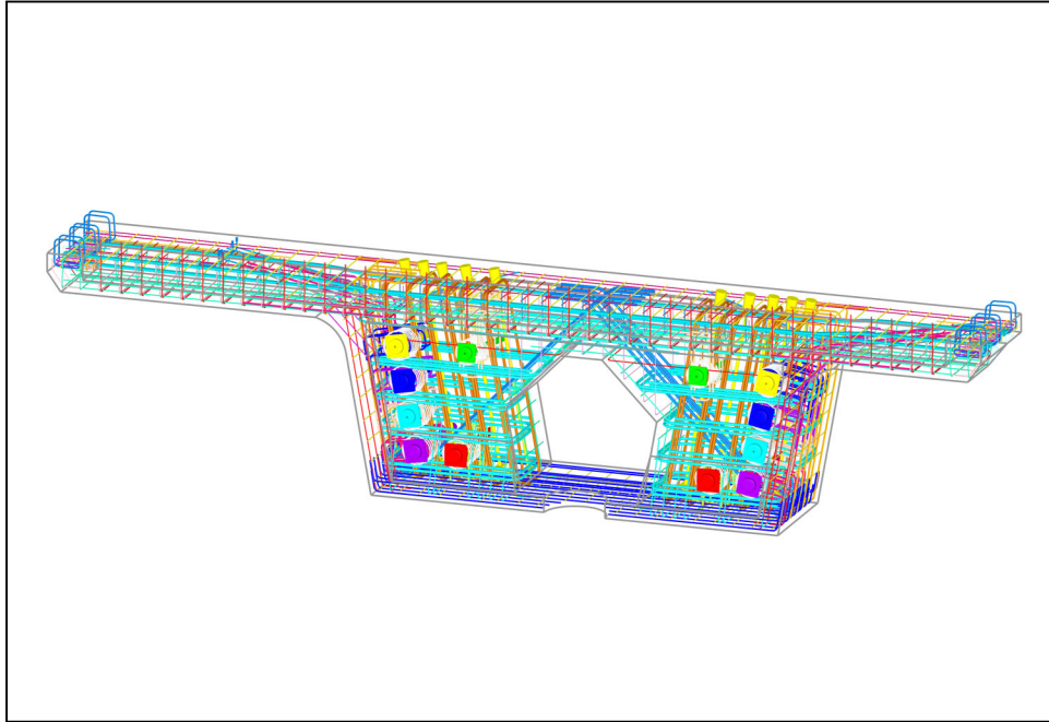
Fig. 2 Example 3-D Color Integrated Drawing
