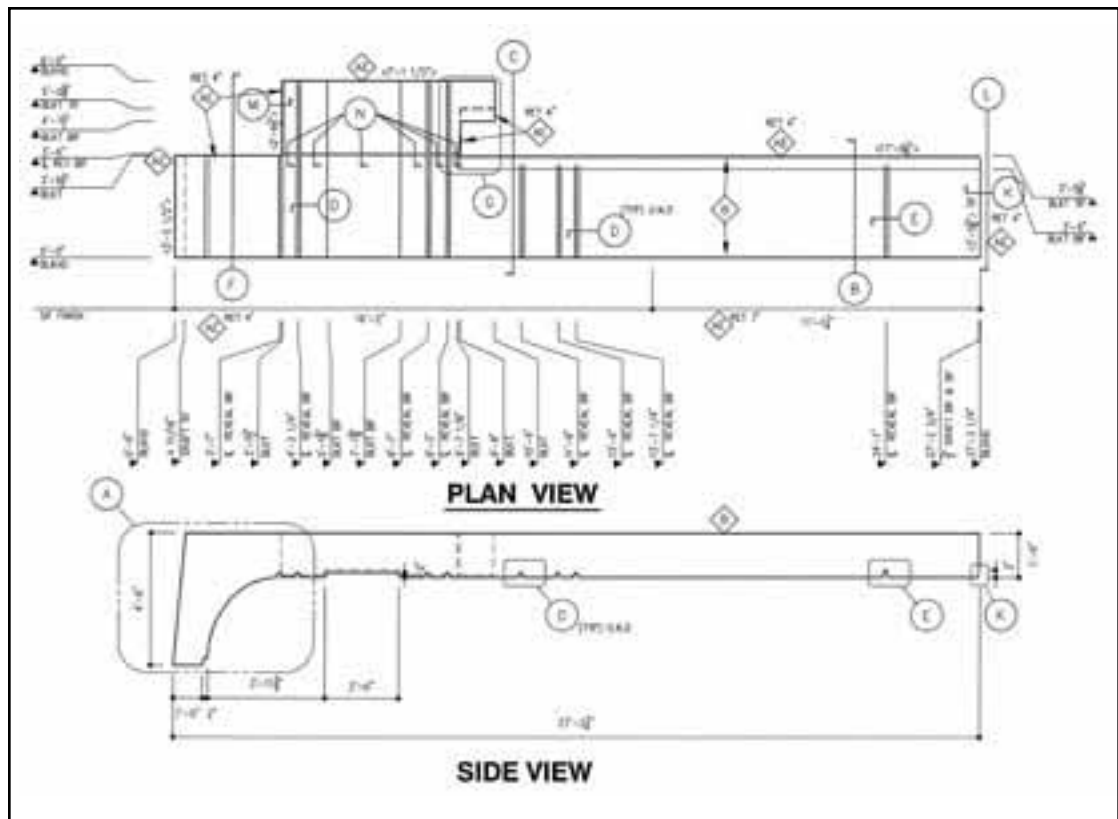
Fig. 14. Plan and side view of typical panel with attached cornice.
